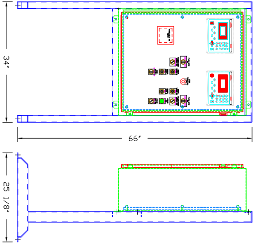
CONTROL ENCLOSURE
